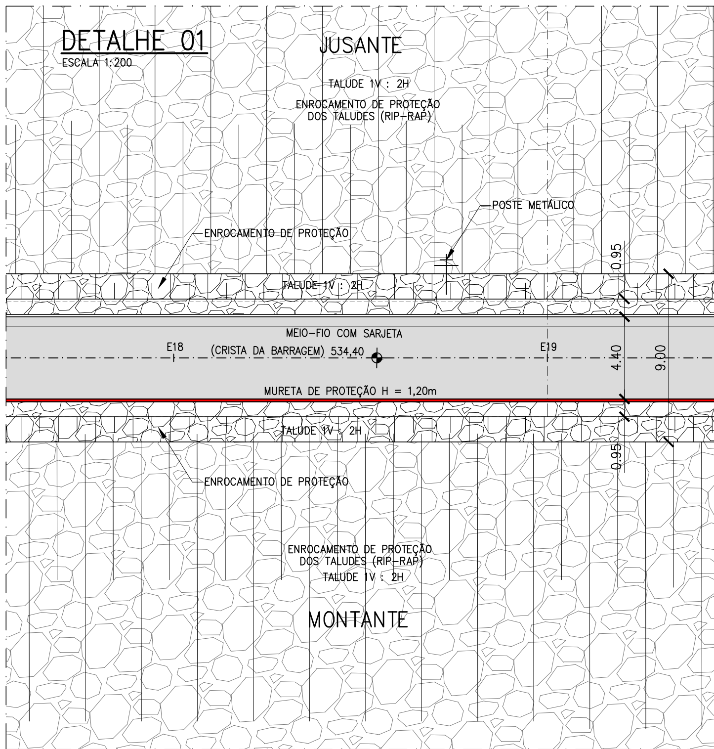
ST-01 (EST. 19+0,00m)
